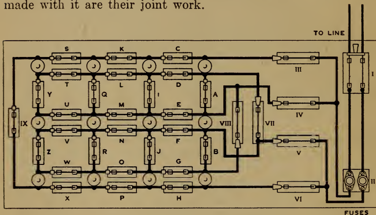
FIG. 3.—A Complex Lamp Bank.
